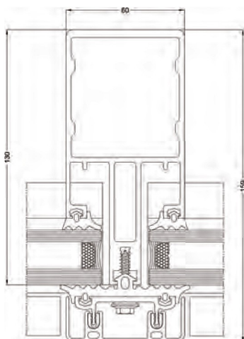
Facciate a copertina Capped curtain walls
